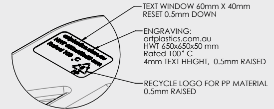
DETAIL D SCALE 1 : 2
